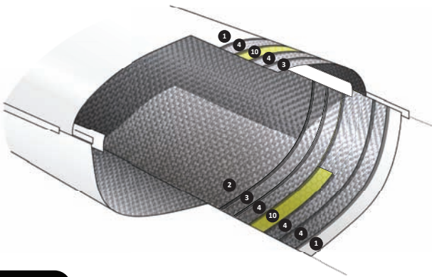
HARDCORE Vacuum deck and hull
