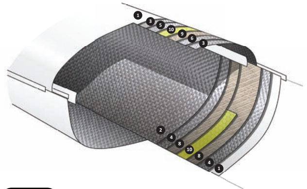
CARBON-PRO Vacuum deck, infused hull
